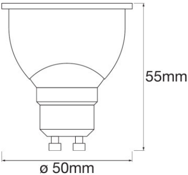
SMART+ WiFi Spot 32 45° 5 W/2700...6500K GU10, SMART+ WiFi Spot 32 45° 5 W/2700...6500K GU10
